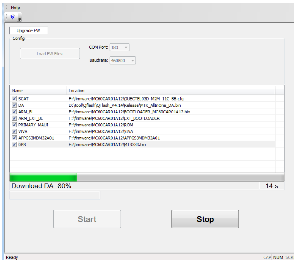
Figure 15: Start Firmware Upgrade after Manually Restarting the Module (M10/M66/M72/M80/M85/M95/MC60/BC660K-GL)
