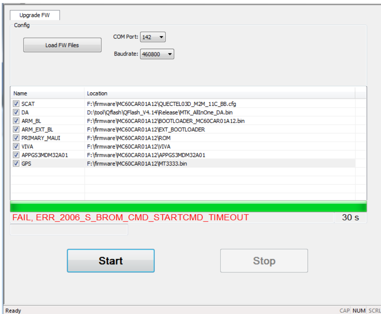
Figure 22: Connected to a Wrong Serial Port (M10/M66/M72/M80/M85/M95/MC60)
