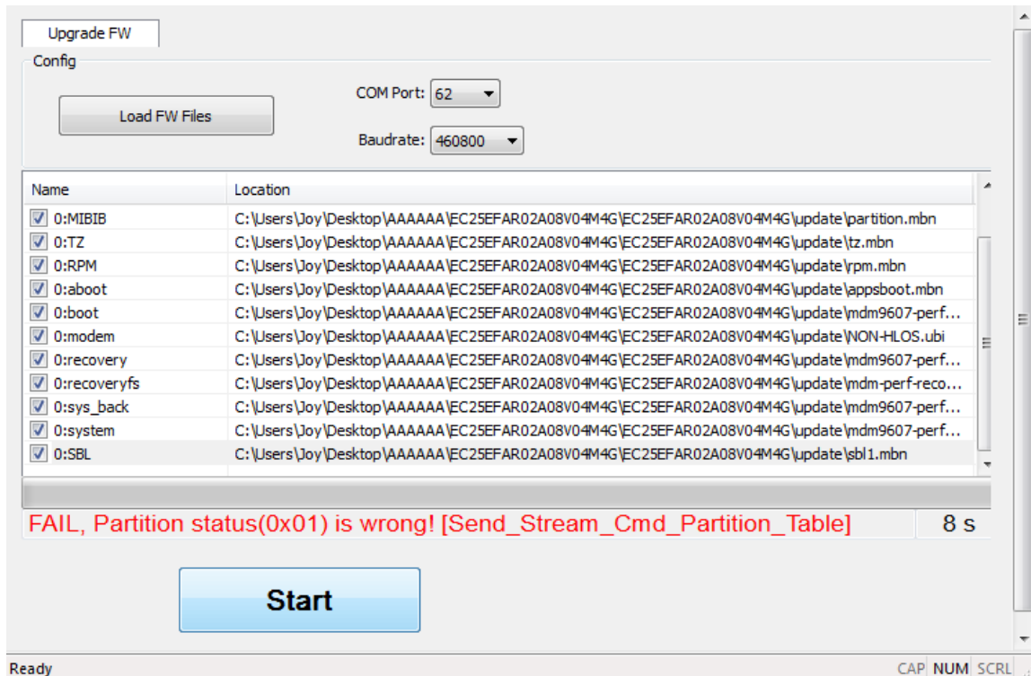
Figure 41: Selected an Invalid FW File (Ex06/AGxx/BG96/EM12)
