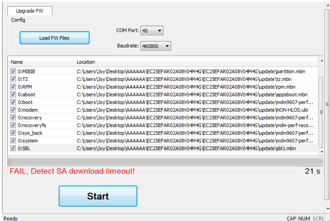
Figure 39: Selected an Invalid FW File (UCxx)
